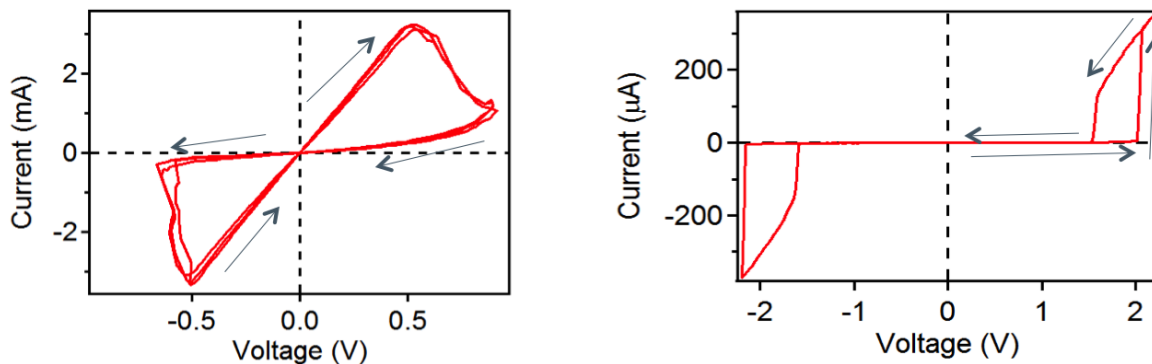
Figure 2: Two types of memristors that could be used in neuromorphic systems [Chua1971, WSP:Williams].
