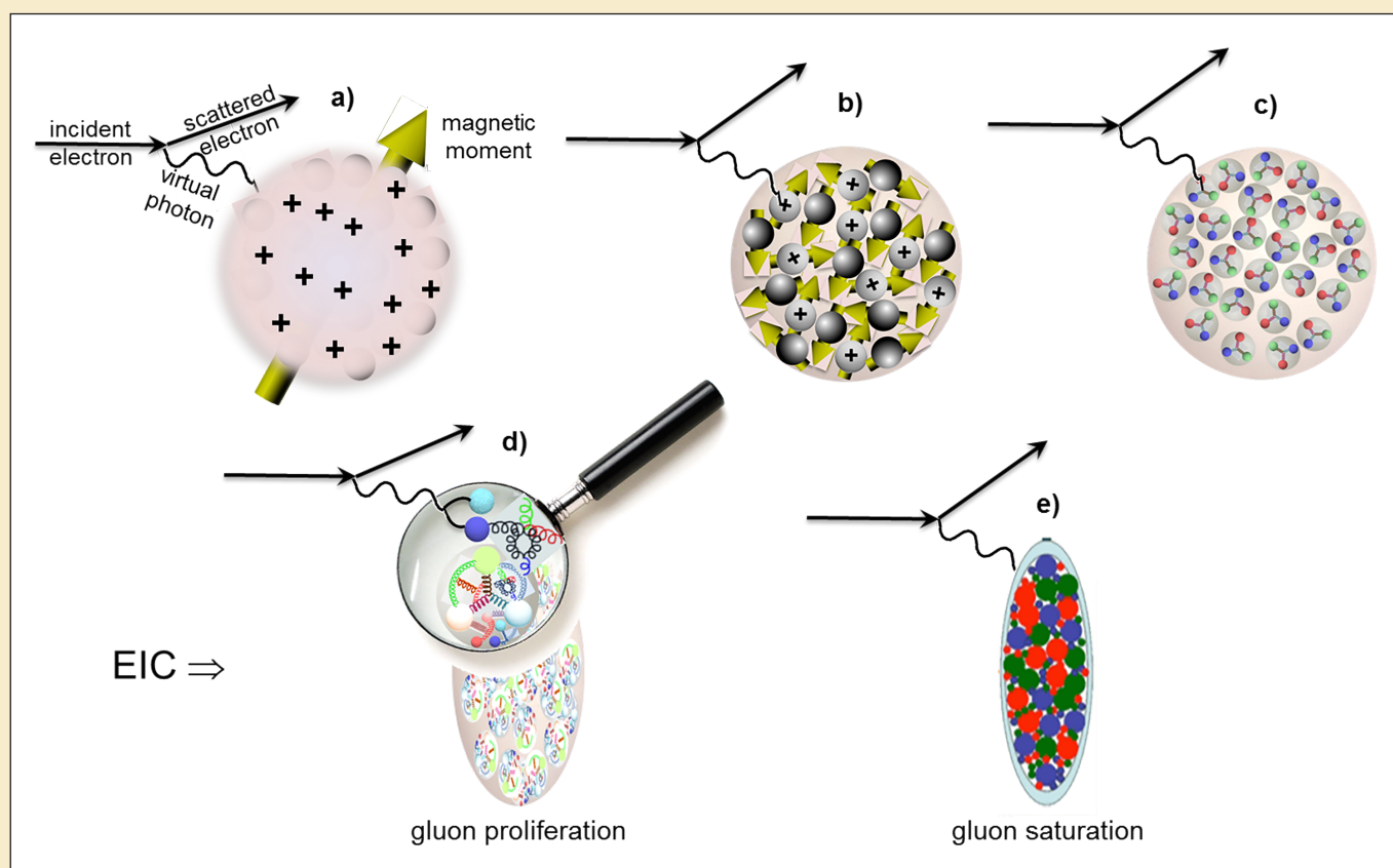
Schematic illustration of the evolving landscape in a nucleus as we alter the resolving power and energy of the electron scattering process used to probe it.
