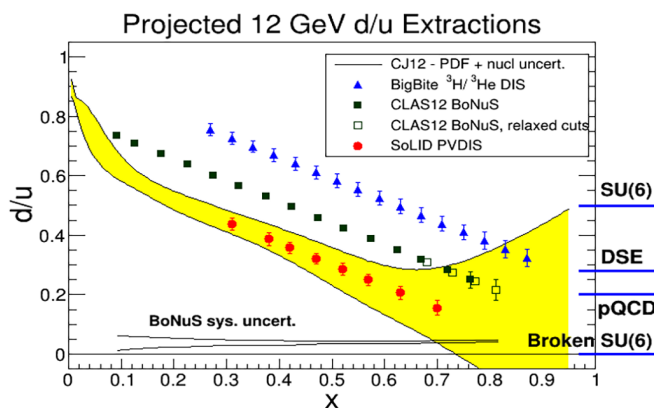
Figure 2.3: Projected uncertainties (offset for display) for JLab 12-GeV measurements of the ratios of the PDFs for the d and u quarks at large momentum fraction x . The yellow band represents the uncertainty in the existing measurements under several theoretical assumptions. Various predictions for this ratio in the limit of x = 1 are given by the blue lines.
