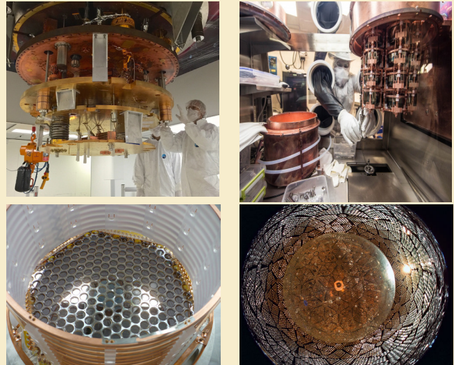
Figure 2: Searches for neutrinoless double beta decay (clockwise from top left) in the coldest space in the universe (CUORE), the cleanest radiation detectors built to date (Majorana), the deepest neutrino detector (SNO+), and the cleanest operational tracking chamber with 3D/time imaging to date (EXO-200).
