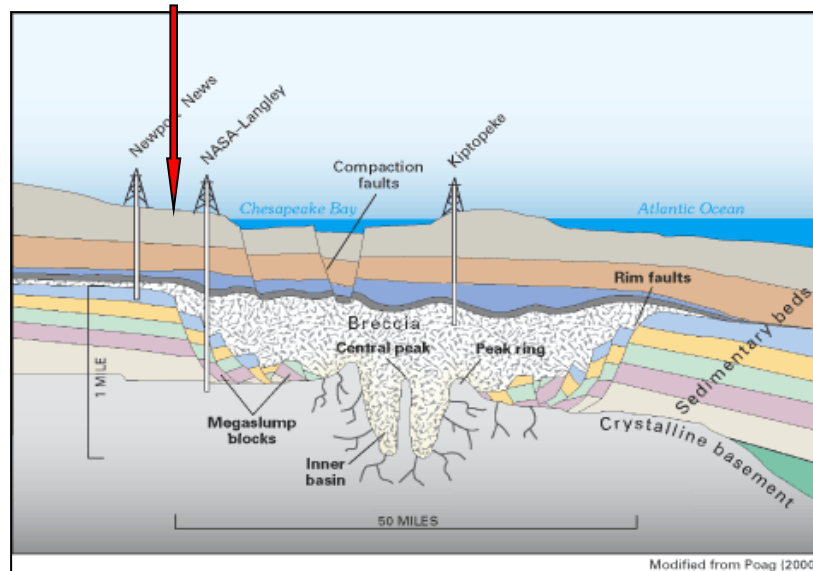
Figure 18 – Location of Jefferson Lab Relative to the Outer Rim of the Chesapeake Bay Bolide Crater
