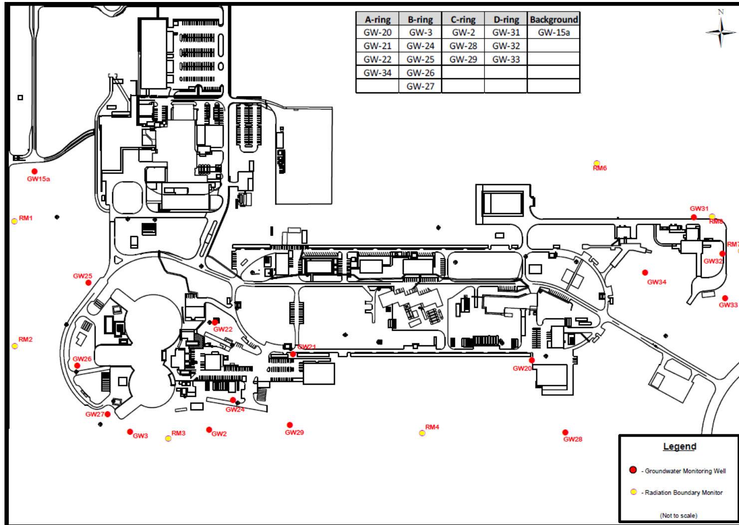
Figure 11 – Radiation Boundary Monitors and Groundwater Monitoring Wells
