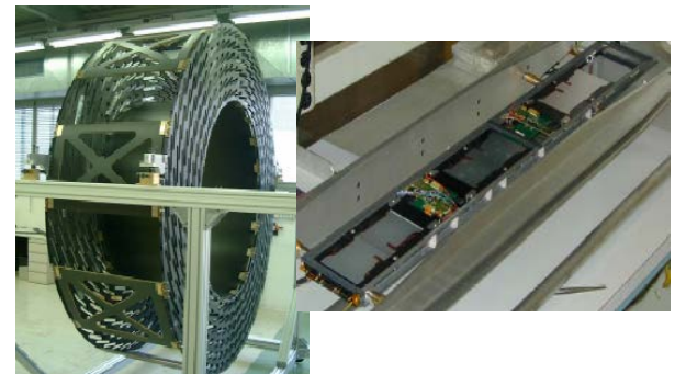
Silicon Tracker Rod Assemblies for Tracker Outer Barrel
