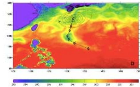
Massive Earth System Model ensembles (e.g. decadal forecasts, extreme weather)
