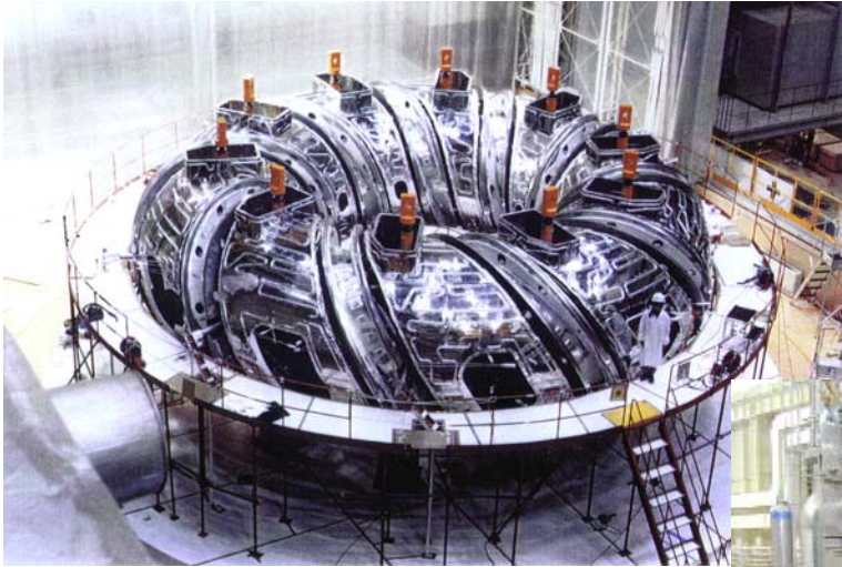
Large Helical Device (LHD)
