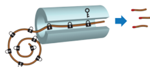
Figure 1. Three mechanistic motifs for polymer upcycling.
