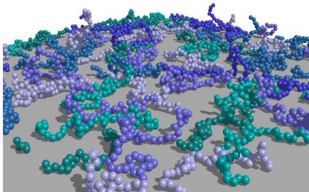
Figure 2. Typical conformation of polymers at a uniformly attractive surface, below the adsorption transition temperature.
