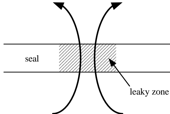
Figure 4 Schematic view of flow self-focusing leading to a reaction-induced breaching of a seal.
