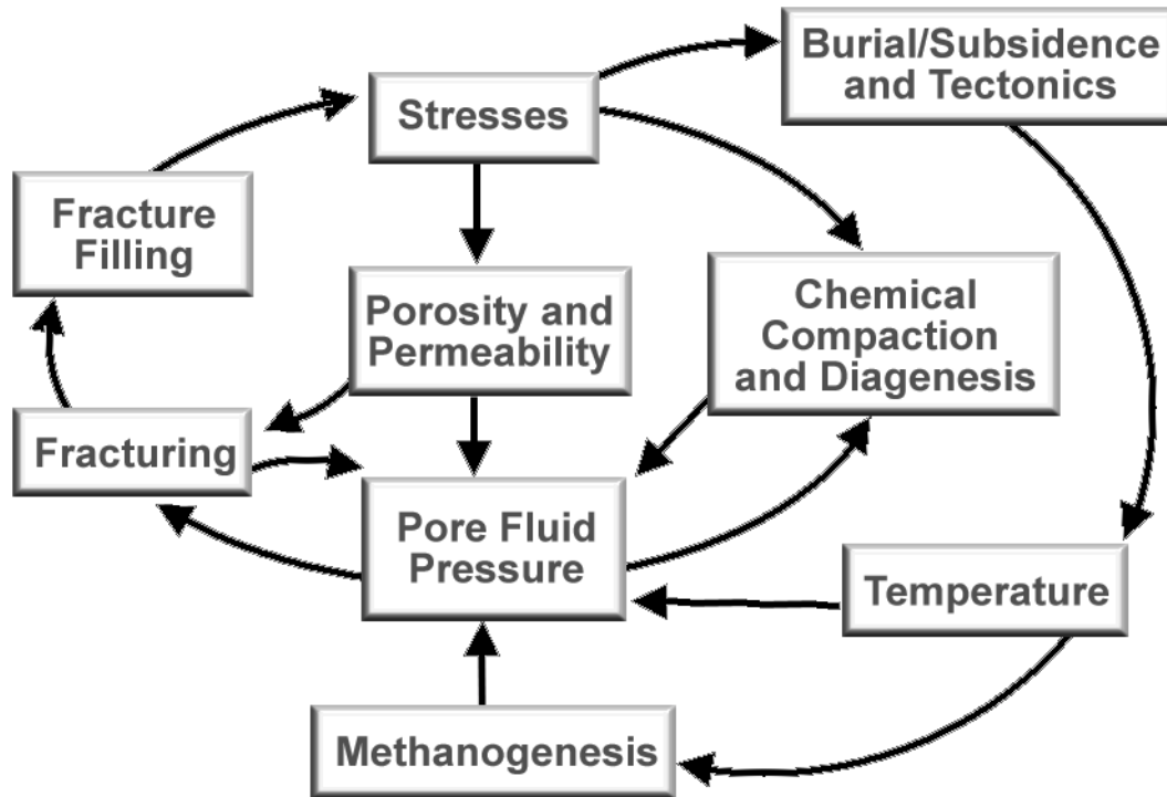
Figure 3 Schematic of parameters and complex feedback between coupled reaction, transport, and mechanical in situ processes
