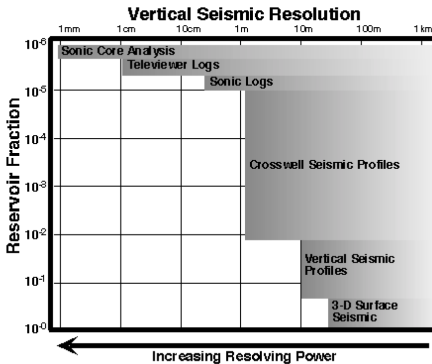
Figure 6 Schematic of seismic resolution versus coverage as a function of seismic method
