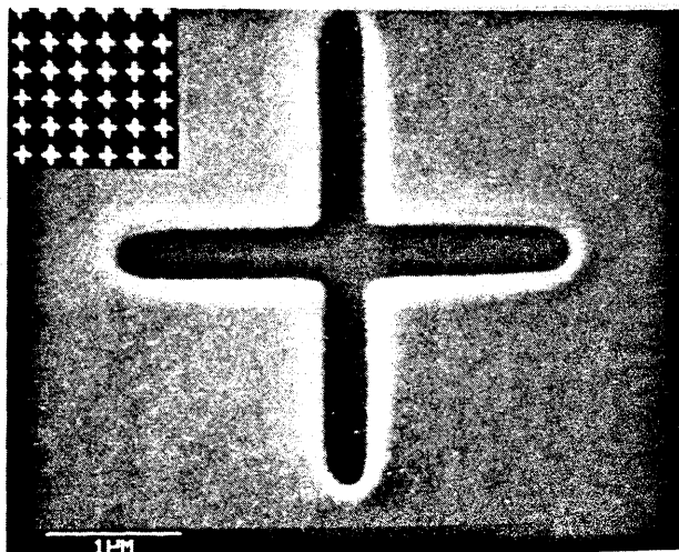
FIG. 2. A small section of an array of resonant elements fabricated at NRRFSS. Enlargements of one element, 3 \mu long, also shown.
