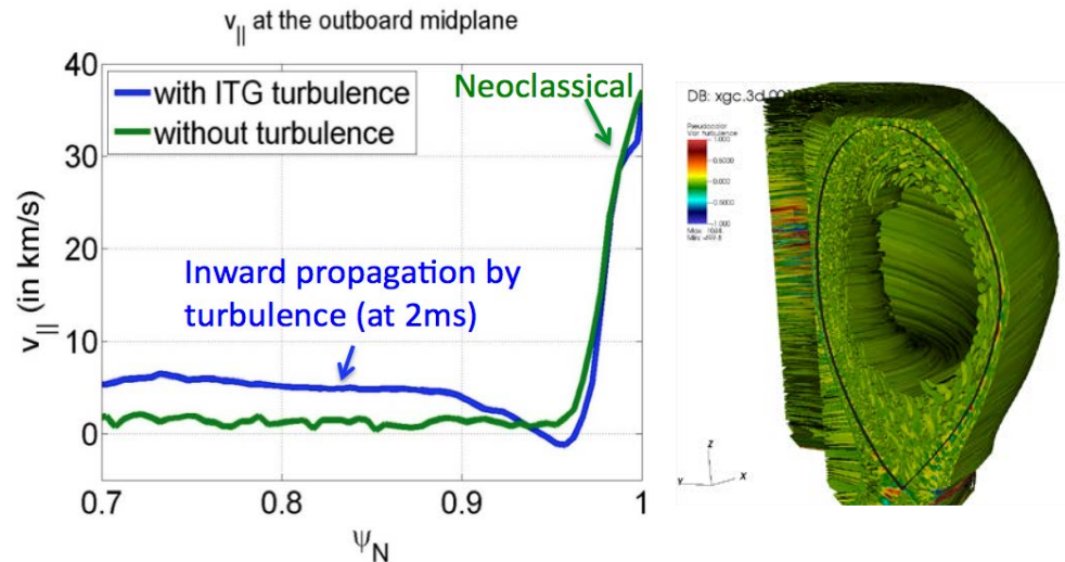
Left: XGC1 identified an intrinsic edge rotation source and an inward momentum pinch phenomenon, similarly to experimental observations Right: Nonlinear coherent turbulence transport momentum inward.
