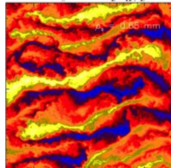
Visualization of small-scale electron temperature fluctuations in the Alcator C-mod tokamak. Note that as the ion sound gyroradius \rho_s = cs/\Omega_{ci} = 0.65 mm in this plasma, the visualization corresponds to a physical domain of approximately 8 mm x 5 mm.
