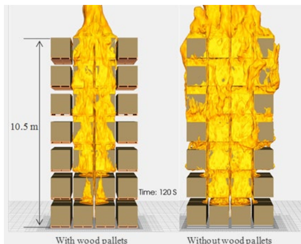
Simulations run on OLCF's Titan shows how stacking commodities on wood pallets (left) slows horizontal fire spread versus absence of pallets (right).
