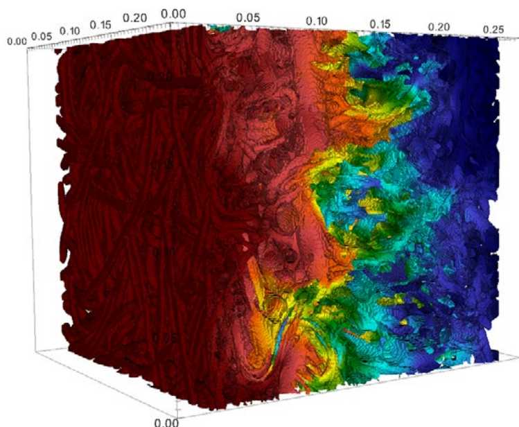
Researchers used a computer simulation framework developed at LLNL that integrates mechanical deformation and two-phase flow models and a full-scale microscale flow model developed at LBNL to model the complex pore structures in the press felts.
