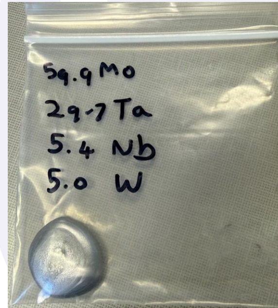
Above, a sample of robotically manufactured AI-optimized material.
