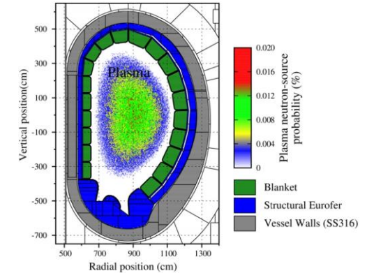
Schematic of a blanket structure surrounding the high temperature plasma in the Commonwealth Fusion Tokamak
