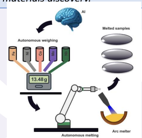
Autonomous arc melting, which Los Alamos has demonstrated, is a step toward physical AI in materials discovery.
