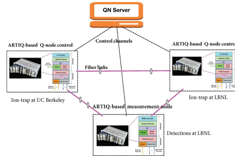
B. Two-level quantum network control
