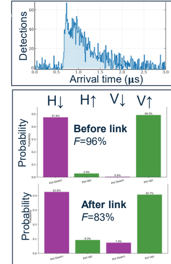
C. Spin-polarization correlations
