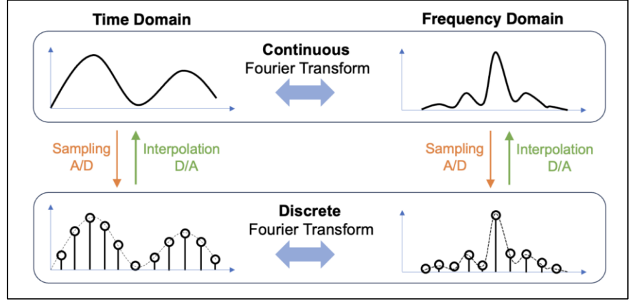
Schematic of classical time-frequency-domain and analog-digital signals, as well as their corresponding Fourier transforms. This work develops the quantum analogues of these protocols---quantum analog-digital conversion protocols---to facilitate quantum signal processing on hybrid quantum processors
