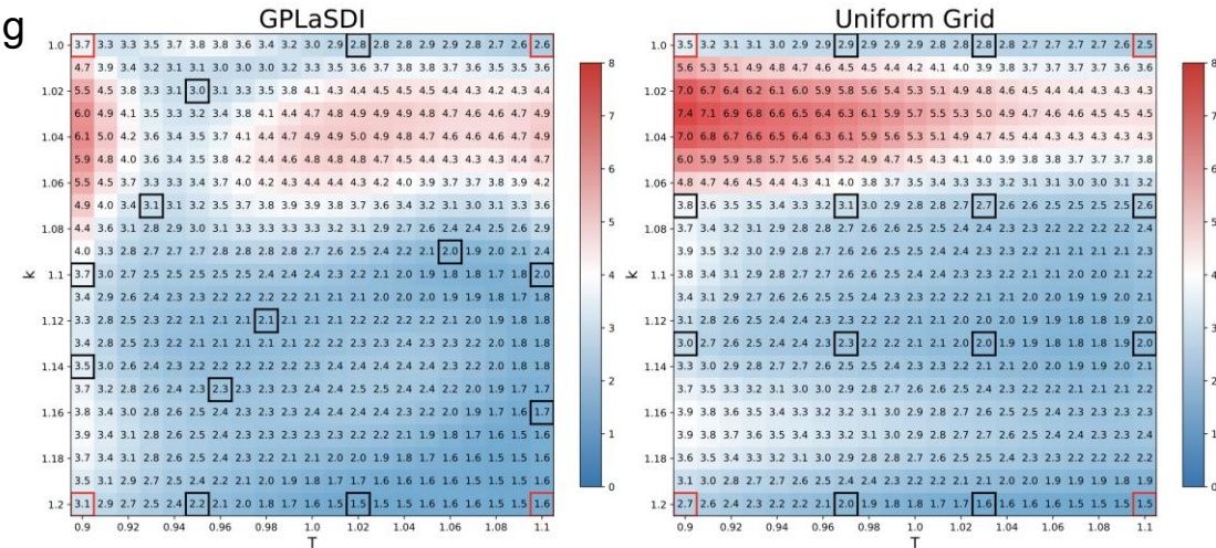
Sampling Comparison. Uncertainty-based sampling (left) and uniform sampling (right)
