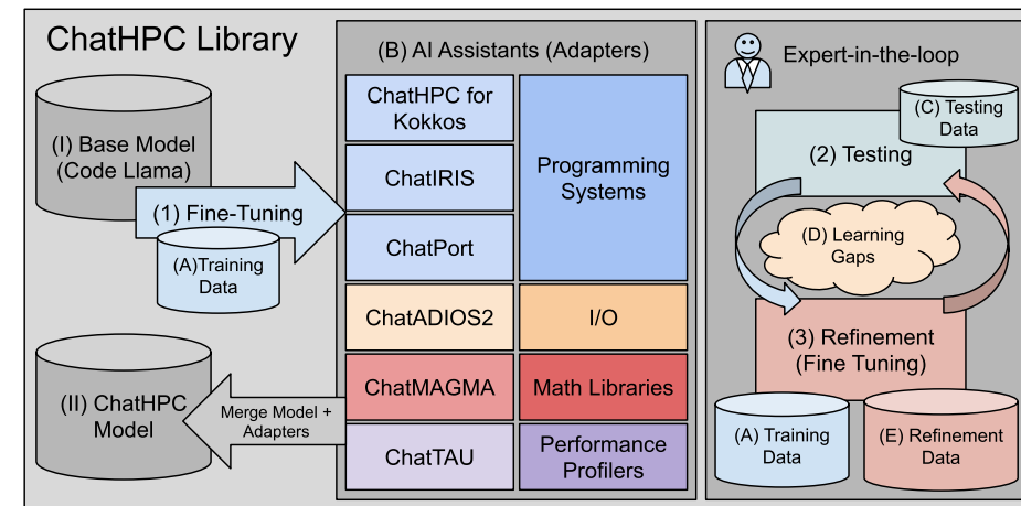
The ChatHPC ecosystem.
