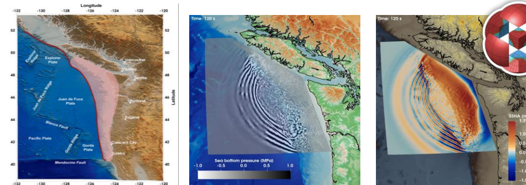
Left: locked part of the plates at the Cascadia subduction zone; Center/Right: sea bottom pressure/surface waves computed with MFEM acoustic-gravity PDE model.
