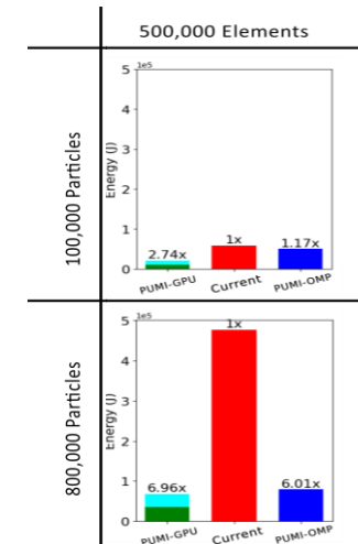
Energy usage for a range of particle counts.
