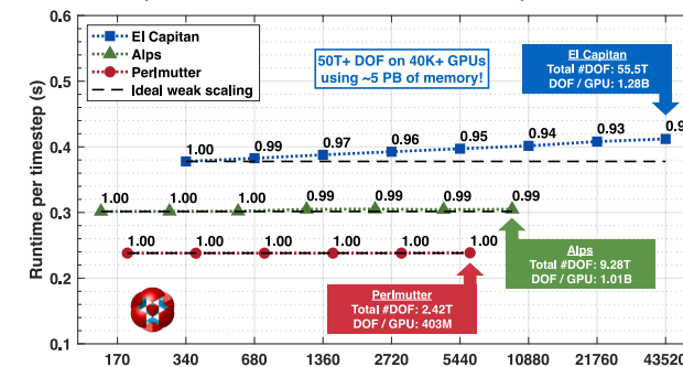
Weak scaling on Perlmutter, Alps and El Capitan, with excellent parallel efficiency up to 55.5 trillion unknowns on 43,520 GPUs (largest FEM simulation ever).
