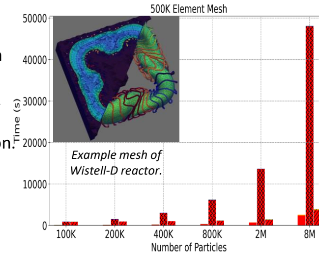
Analysis runtime comparison of current OpenMC approach and PUMI-Tally based approach.
