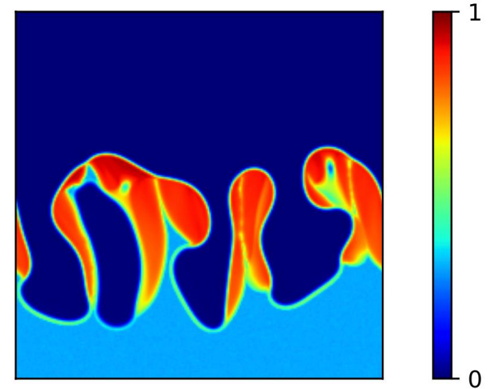
Metal composition profile at the micro-scale. Dark blue represents a molten corrosive salt, and light blue represents (sane) metal, for instance a Chromium-Nickel alloy. At the micro-scale, the metal surface will deform, and the salt may poke holes in the metal. The Chromium concentration spikes at the salt-metal interface, indicating de-alloying patterns (and thus degraded material properties)
