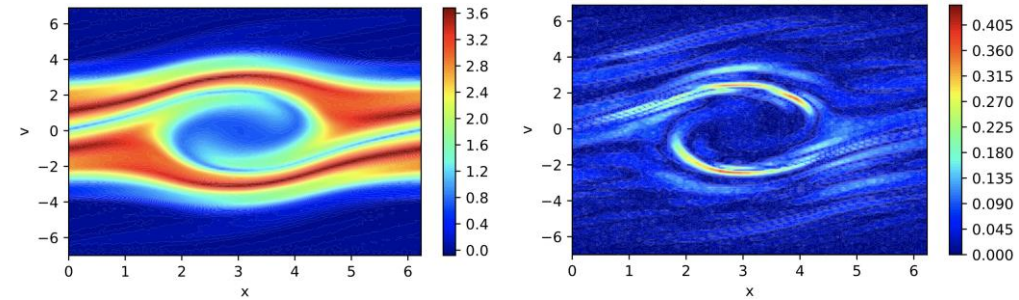
Test Problem. 1D1V Vlasov two stream instability; GPLaSDI prediction (left) and Absolute error (right)
