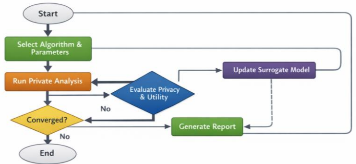
Figure 1: Overview of PRESTO's modular framework.
